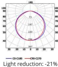
PHOTOMETRIC CURVE
