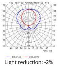
PHOTOMETRIC CURVE
