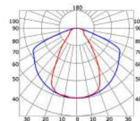
60° lens cover (light reduction: -3%)
