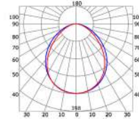
Semiopal cover (light reduction: -9%)
