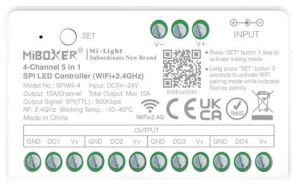
SPIW5-4 4-Channel 5 in 1 SPI LED Controller WiFi + 2.4G RF
