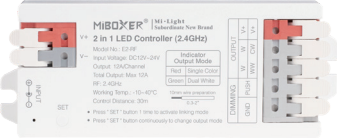
E2-RF 2 in 1 LED Controller (Single Color / Dual White)
