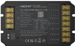
HZ5 5 in 1 LED Controller (Single Color / Dual White / RGB / RGBW / RGB+CCT)
