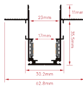
20 Style Flush Mounted Magnetic Rail Model No.: AM-MR-20F15B (1m) Model No.: AM-MR-20F15C (2m)
