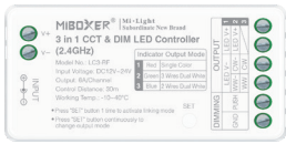
LC3-RF 3 in 1 CCT & DIM LED Controller (Single Color / 3 Wires Dual White / 2 Wires Dual White)
